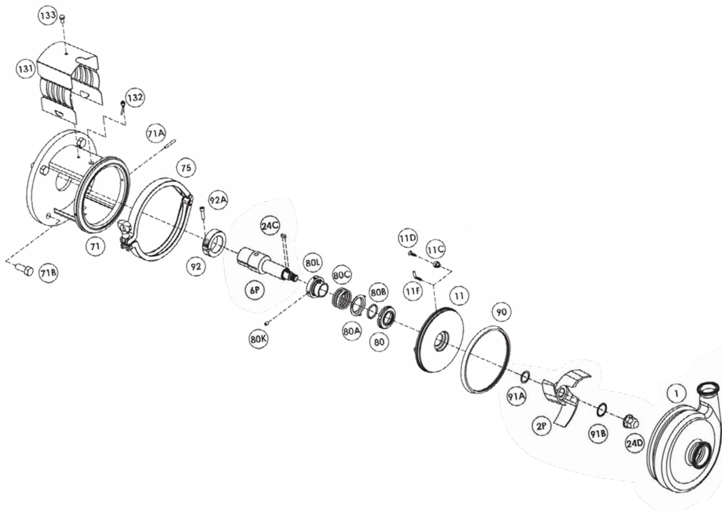
Figure 5: Expanded View
